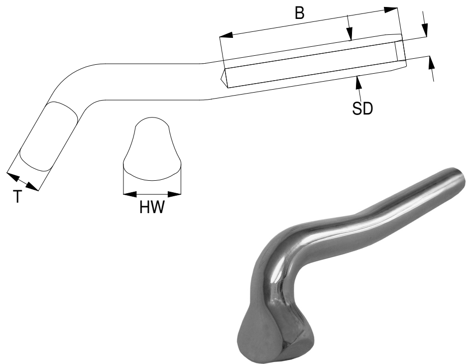
Shroud Terminals for Metric Wire
